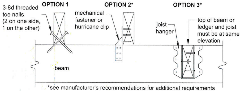
Figure 6. Joist-to-Beam Detail.
