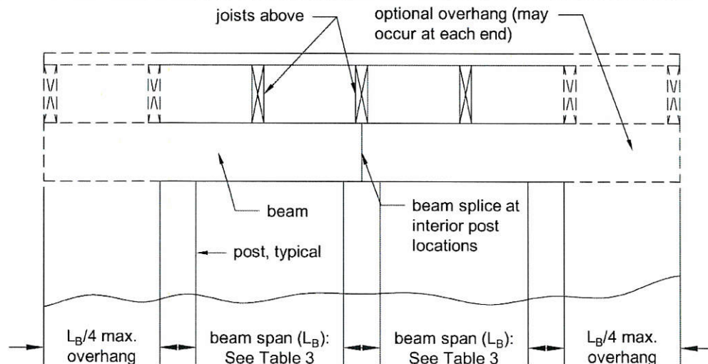
Figure 3. Beam Span.
