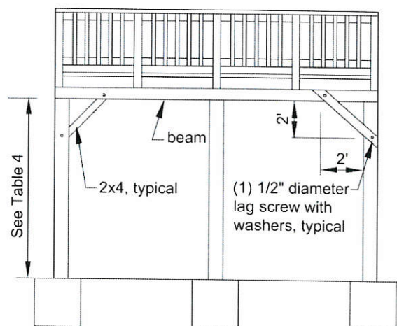
Figure 10. Diagonal Bracing.
